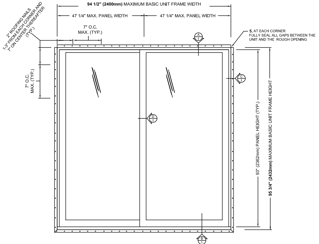
ELEVATION SHOWING FASTENER LOCATION & SPACING
